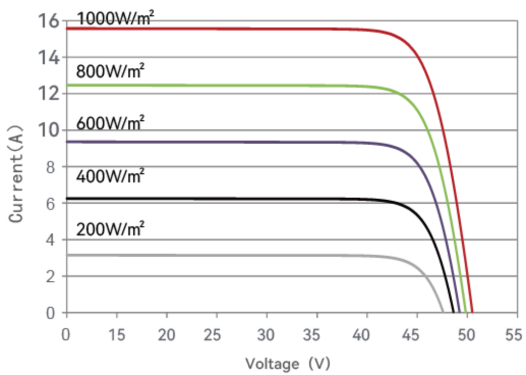
I-V curve
