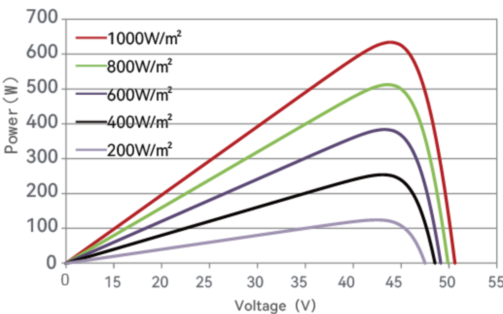
P-V curve
